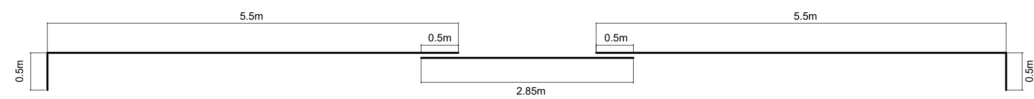
3 Section Rebar Overlap Detail, Typ. 1:50
