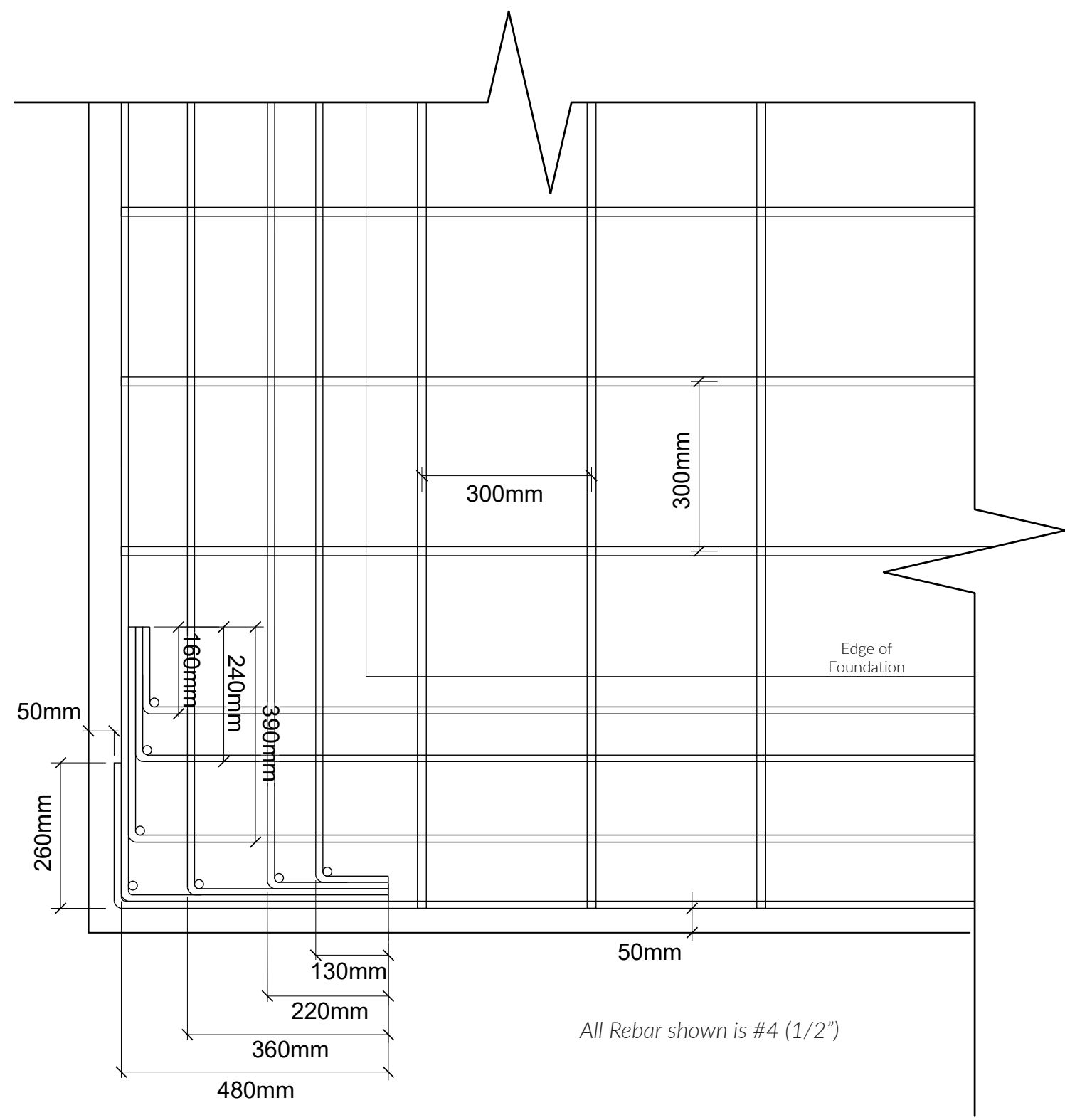
2 Plan Slab Corner Detail 1:10
