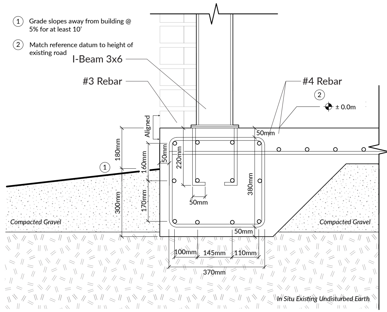
1 Section Column @ Foundation 1:10
